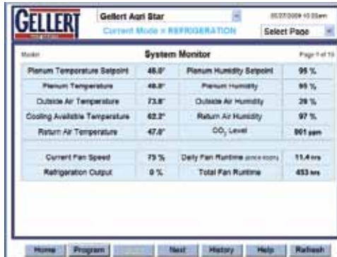
System Monitor
